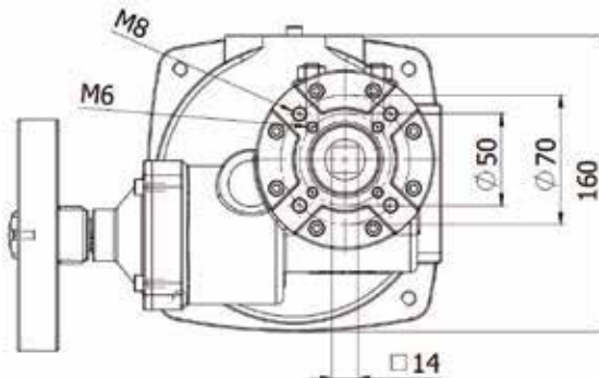
Figure 4. ISO 5211 Sizes
